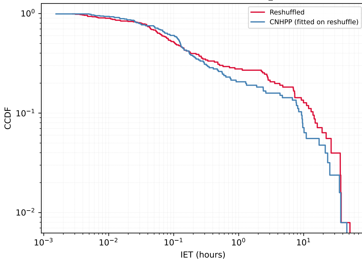
User 7567764882 - Reshuffled vs CNHPP A_{\text{fit}}=0.4688
